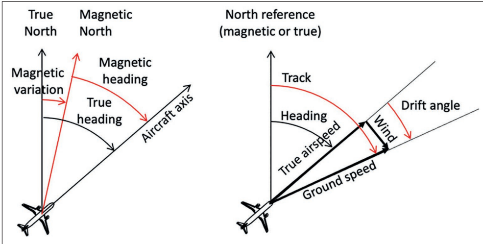
Figure 2: Heading and track information.
