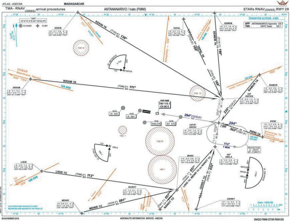
Figure 10: Arrival chart (RNAV STARS) for runway 29 in Antananarivo (FMMI), published by ASECNA: courses between WPTs are published in magnetic and true reference. © ASECNA
