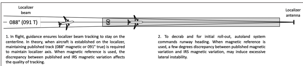
Figure 5: ILS approaches.
