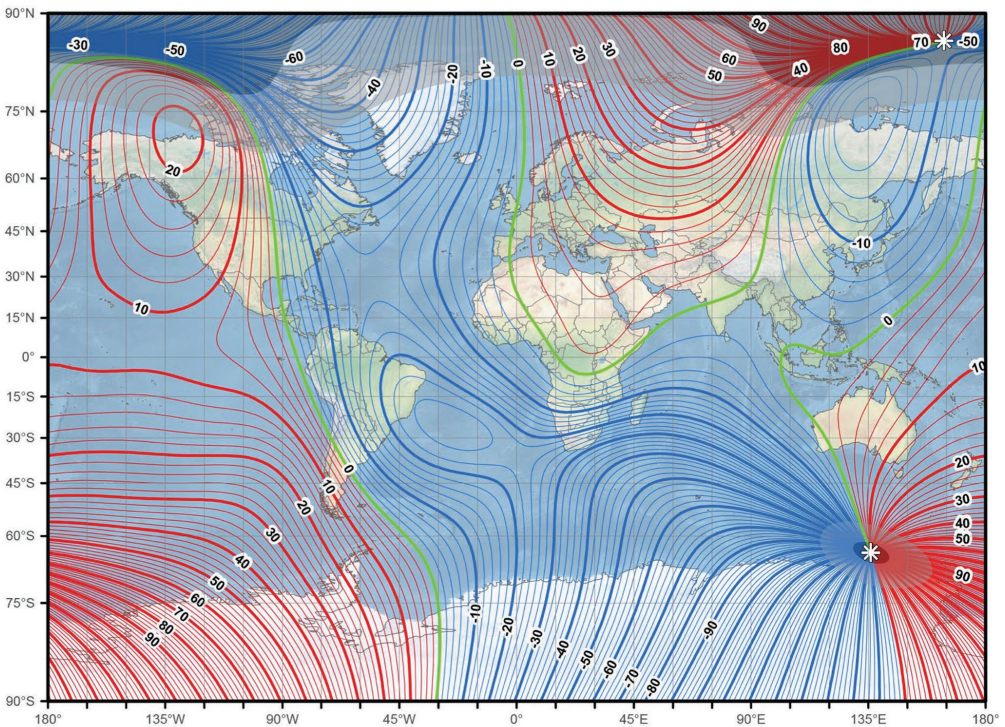
Figure 1: Constant magnetic variation lines from WMM 2020 model. Red contours positive (east); blue negative (west); green zero (agonic) line. Magnetic poles (dip poles) are represented by white star symbols. © NOAA/CEI
