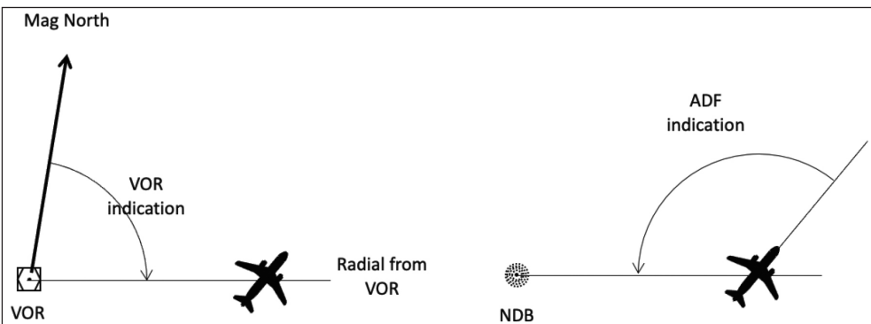
Figure 7: VOR receivers.
