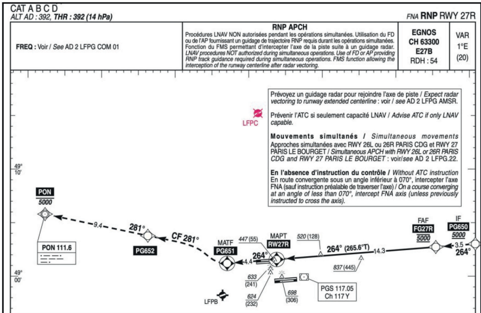
Figure 9: Final approach chart for RNP RWY 27R approach (LFPG - Paris CDG).
